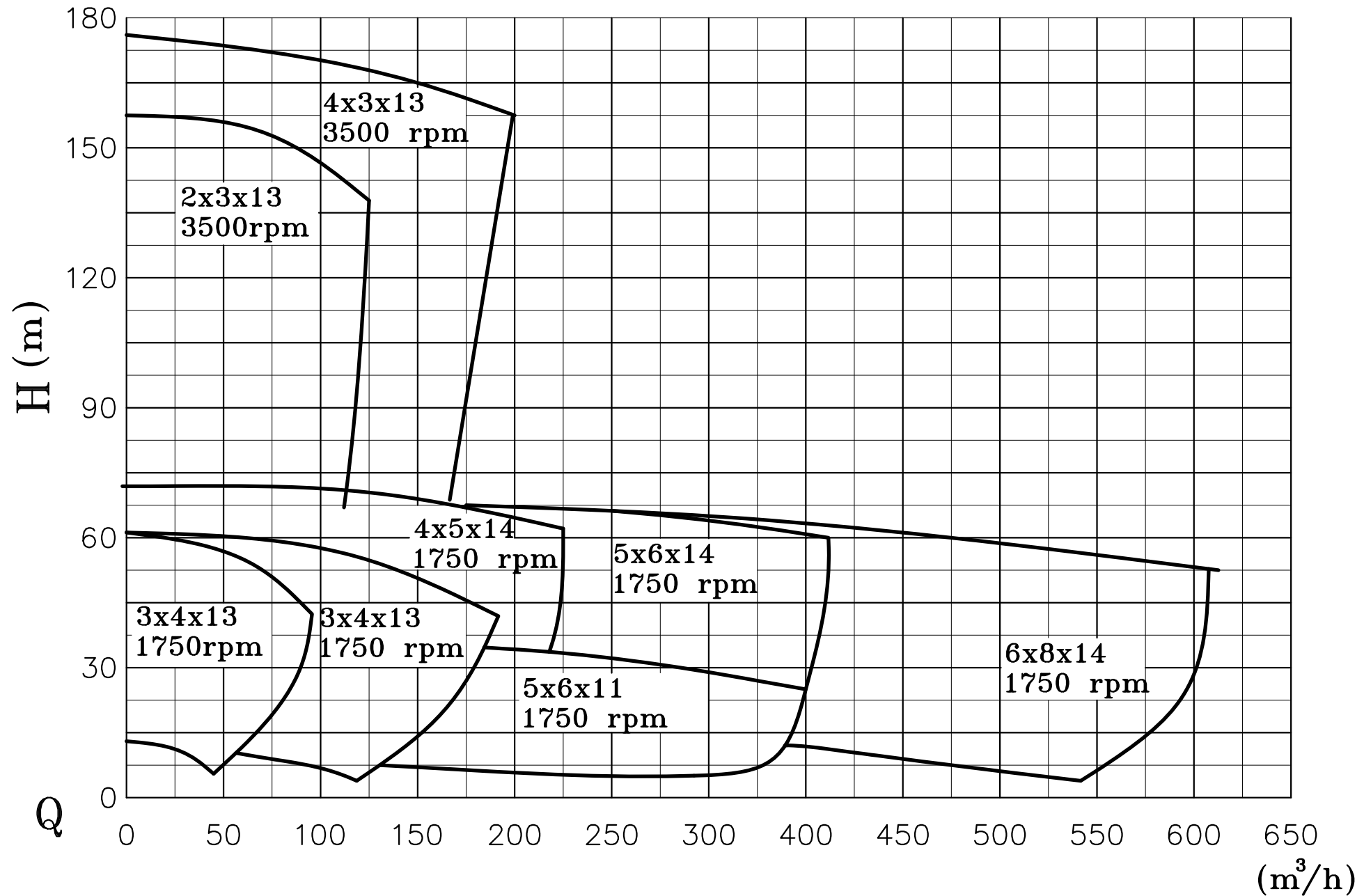
Performance curves - 60 HZ
