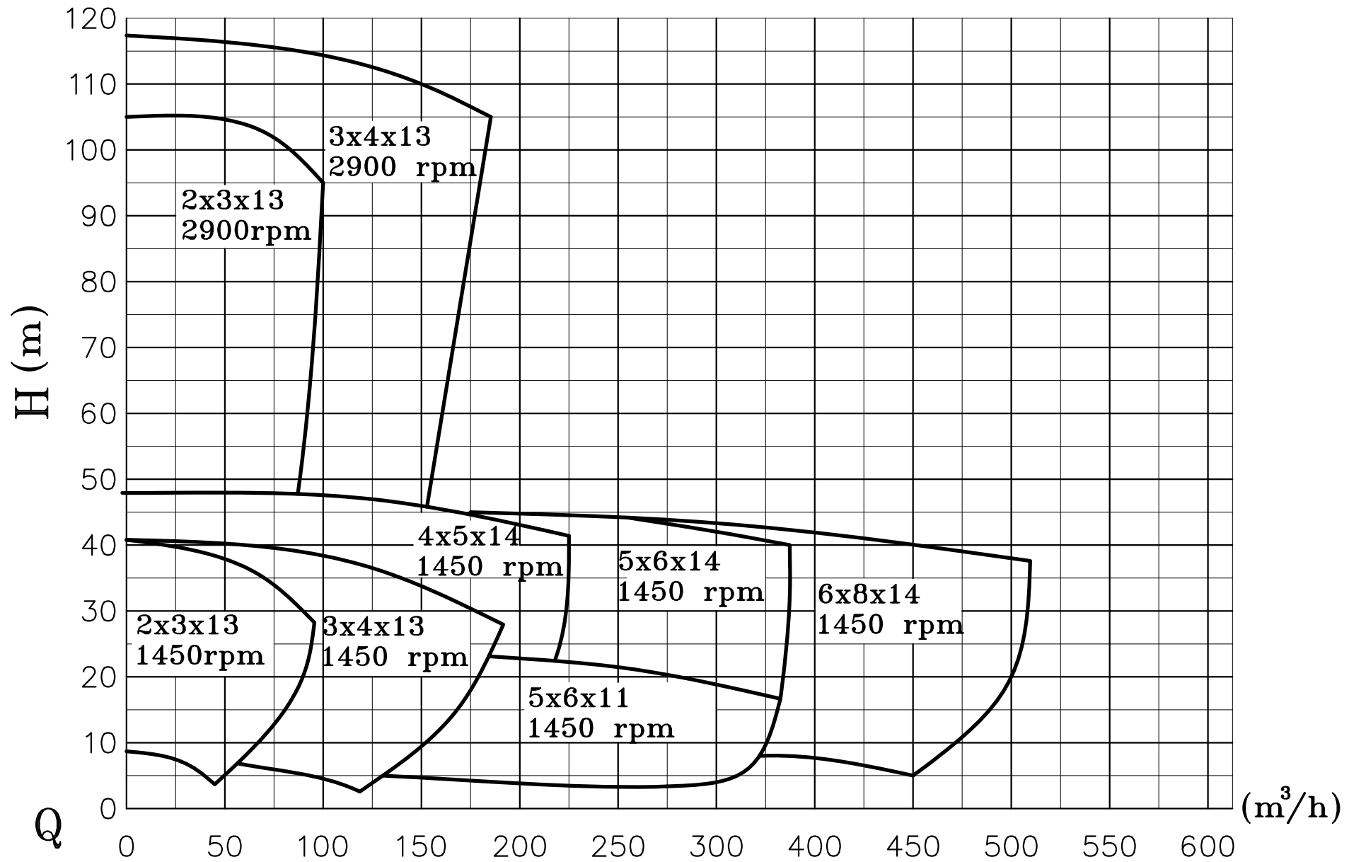
Performance curves - 50 HZ
